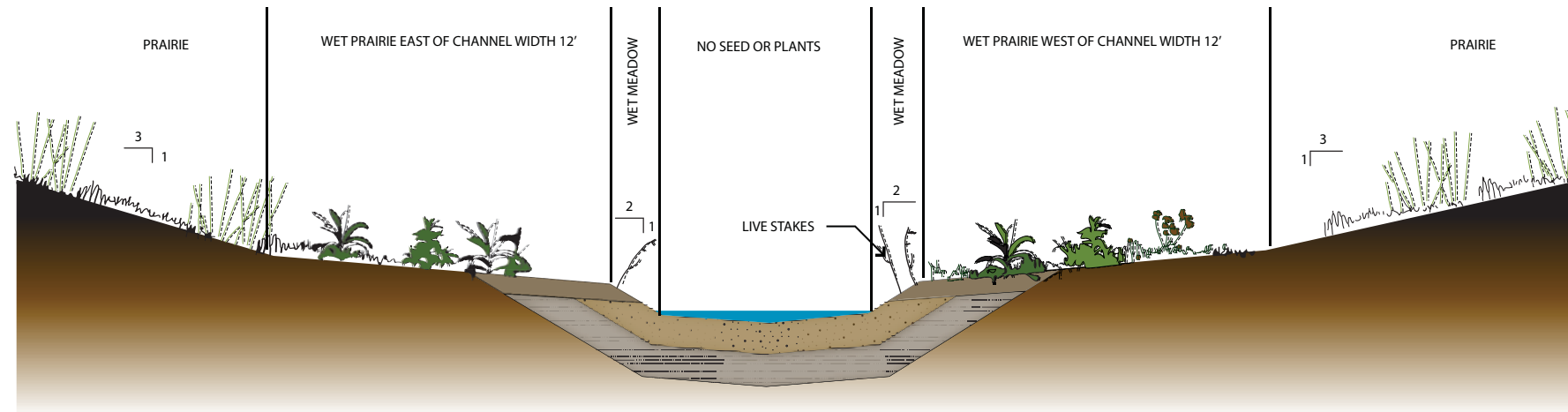
TYPICAL SECTION: TROUT BROOK CHANNEL
