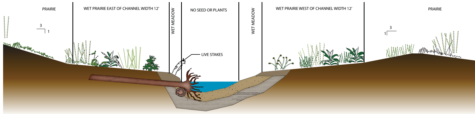
TYPICAL SECTION: TROUT BROOK CHANNEL WITH LARGE WOODY DEBRIS
